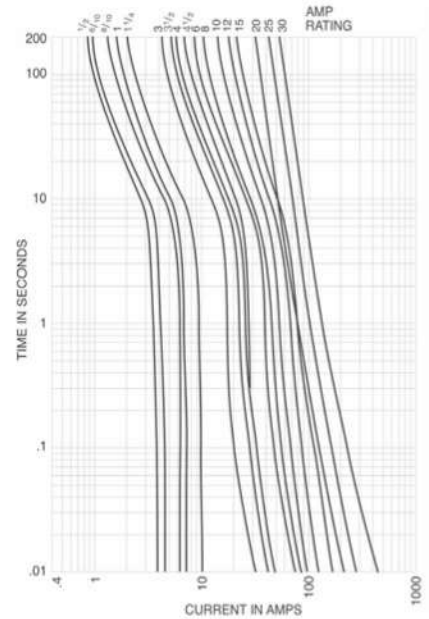
Time-current characteristics-average melt
