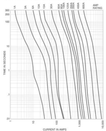
Time-current characteristic curves-average melt
