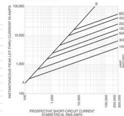
Current limitation curves
